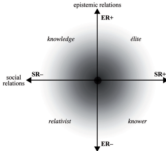
Figure 1: Specialization plane
